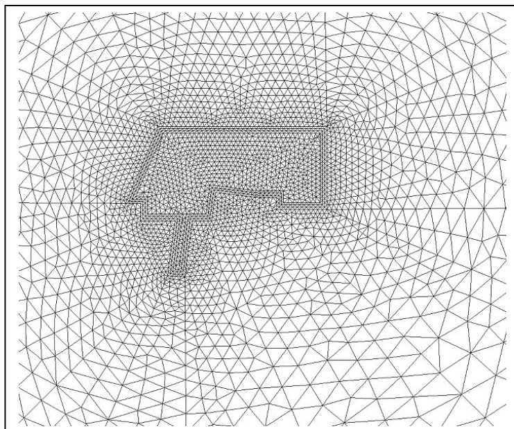
Fig. 1 Part of a finite-element grid for a construction dewatering.
